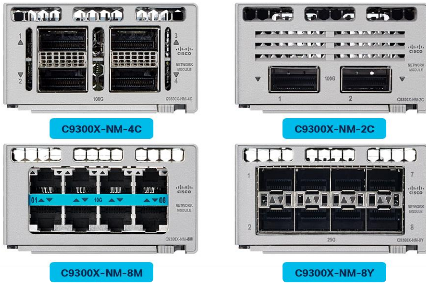
Figure 2. Cisco Catalyst 9300X Network Modules
